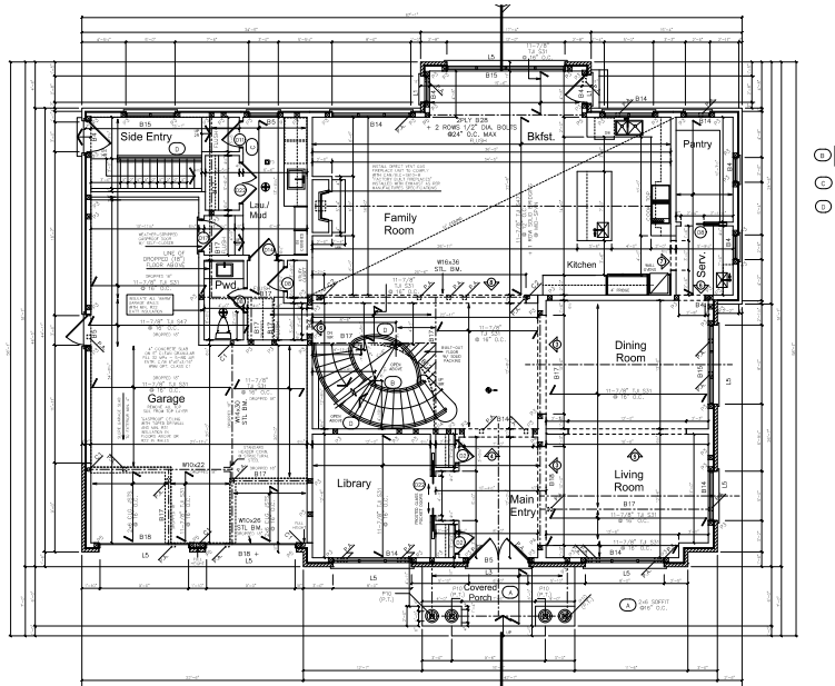
Lower Level - 2,443 sq.ft.
