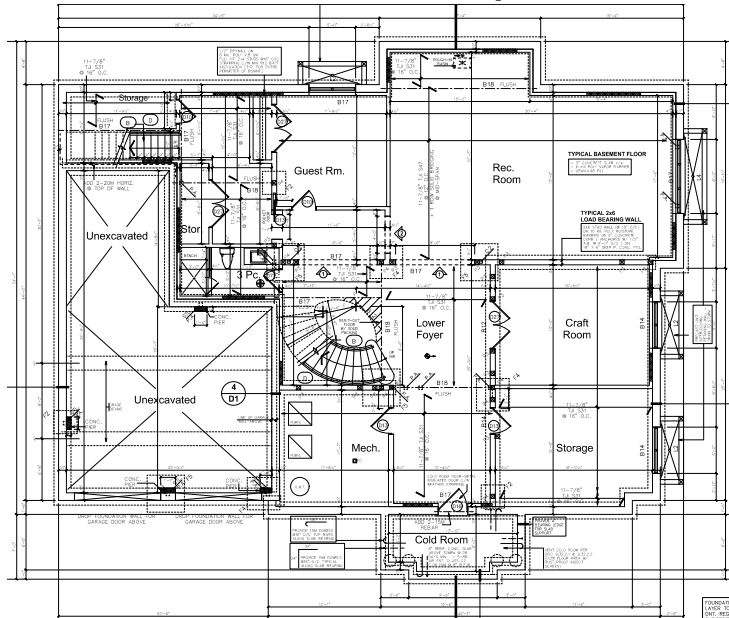
Lower Level - 2,443 sq.ft.
